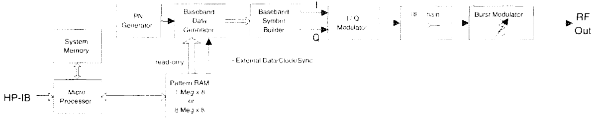
Figure 3-1 HP ESG-D and HP ESG-DP Series Signal Generator Option UN8/9 Modulation Block Diagram
