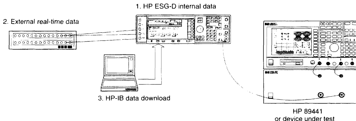
Figure 3-3 HP ESG-D and HP ESG-DP Series Signal Generator Data Sources
