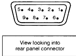
Figure 2-2 The Signal Generator’s AUXILIARY INTERFACE (RS-232) Connector
