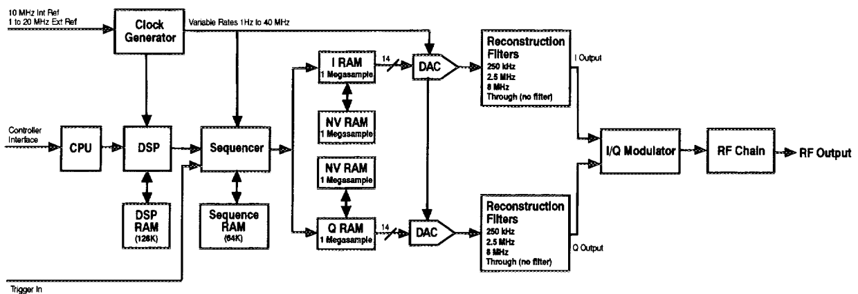
Figure 3-2 HP ESG-D and HP ESG-DP Series Option UND Modulation Block Diagram
