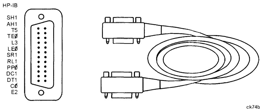
Figure 2-1 HP-IB Connector and Cable
