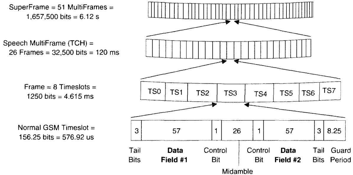
Figure 5-1 GSM Multiframe Transmission
